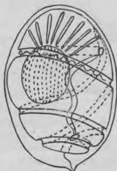
Fig. 5. Cochlodinium radiatum KOFOID and SWEZY. View of right side. Original, Asamushi, 1930. \times 800 .
