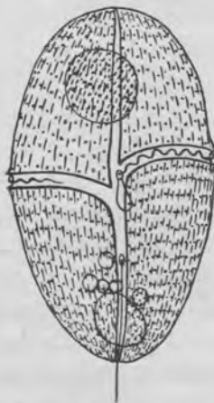
Fig. F. Gymnodinium heterostriatum KOFOID and SWEZY. Ventral view. After KOFOID and SWEZY (1921, Fig. Y, 7). \times 800 .
